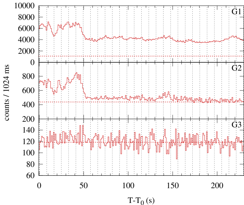
Konus-WIND S2 SOL2000-06-17T02:31 (M3.5) T 0 = 9065.676 s UT (02:31:05.676)
