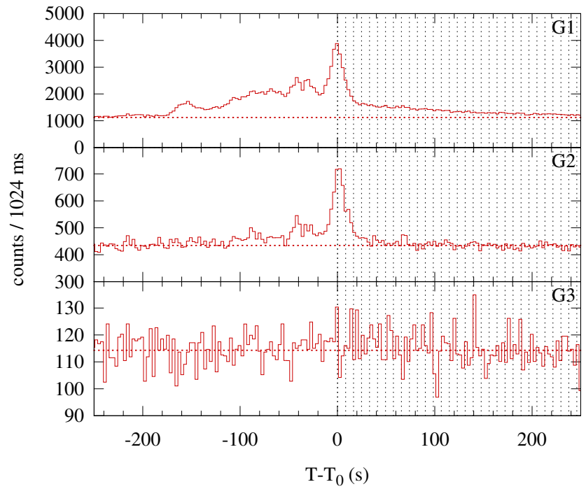
Konus-WIND S2 SOL2000-07-10T20:00 (M1.9) T 0 = 72057.536 s UT (20:00:57.536)
