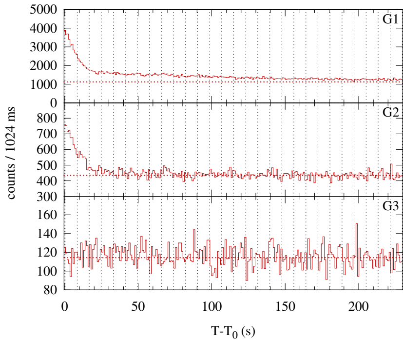
Konus-WIND S2 SOL2000-07-10T20:00 (M1.9) T 0 = 72057.536 s UT (20:00:57.536)
