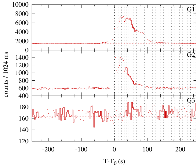
Konus-WIND S2 SOL2000-07-12T21:39 (M1.9) T 0 = 77957.28 s UT (21:39:17.28)
