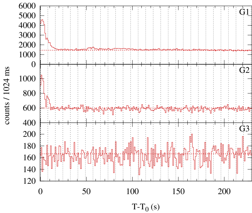
Konus-WIND S2 SOL2000-07-13T16:17 (M1.1) T_0 = 58663.205 s UT (16:17:43.205)
