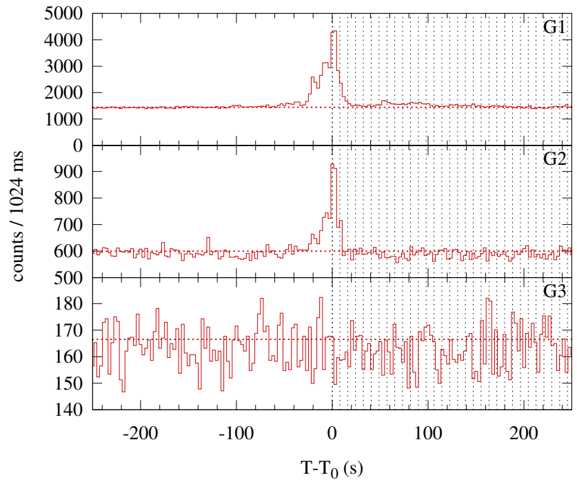
Konus-WIND S2 SOL2000-07-13T16:17 (M1.1) T_0 = 58663.205 s UT (16:17:43.205)
