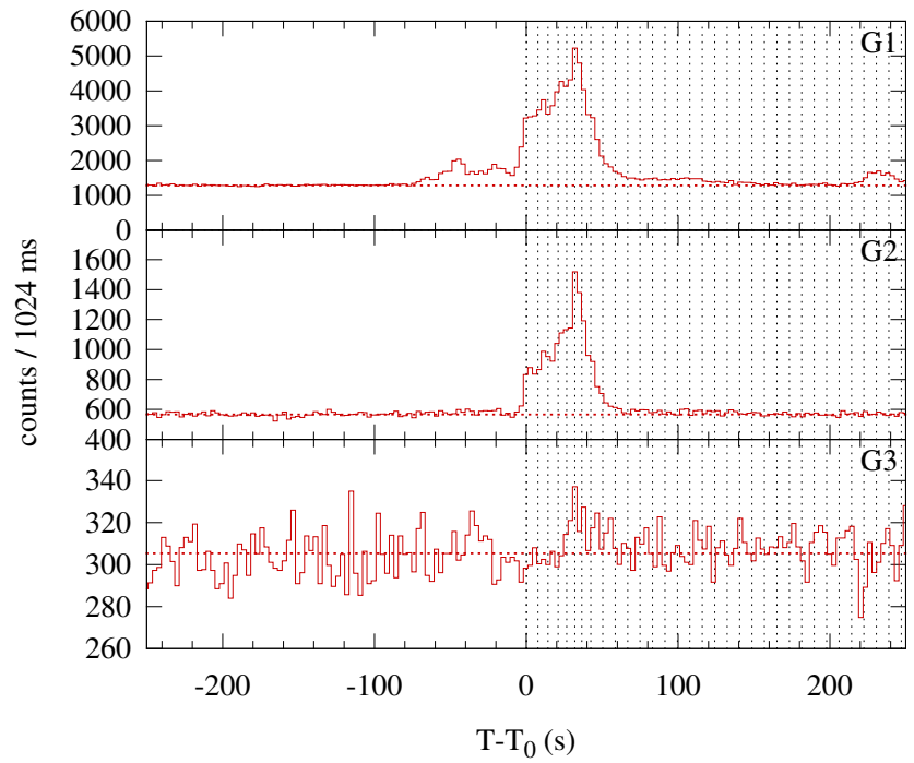
Konus-WIND S2 SOL2000-07-25T18:44 (M1.2) T_0 = 67473.865 s UT (18:44:33.865)
