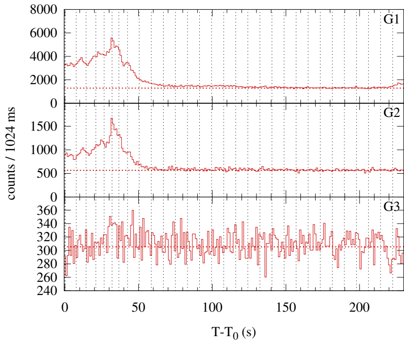
Konus-WIND S2 SOL2000-07-25T18:44 (M1.2) T_0 = 67473.865 s UT (18:44:33.865)
