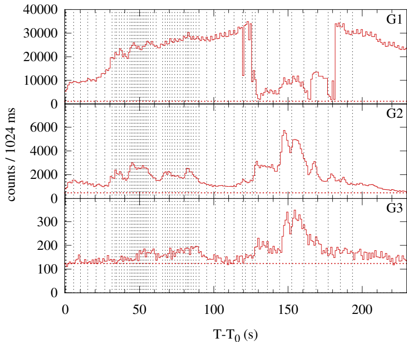
Konus-WIND S2 SOL2000-09-30T23:16 (X1.2) T_0 = 83813.979 s UT (23:16:53.979)
