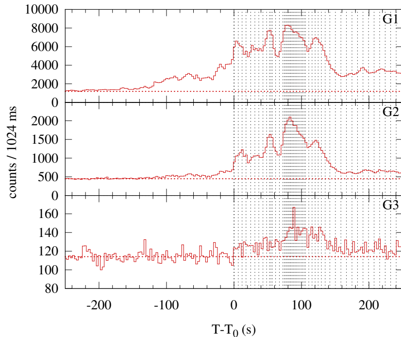
Konus-WIND S2 SOL2000-10-29T01:45 (M4.4) T_0 = 6346.243 s UT (01:45:46.243)
