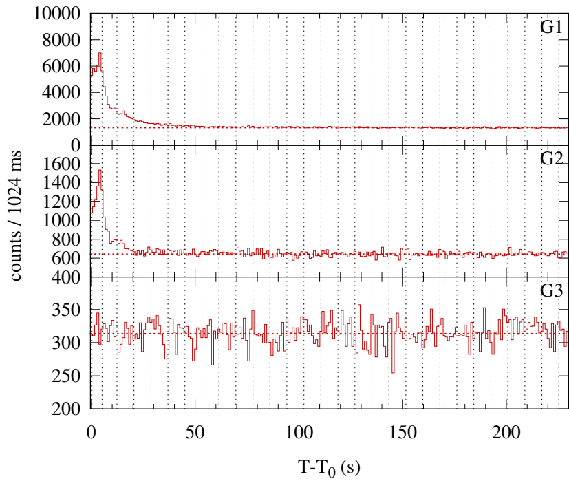
Konus-WIND S2 SOL2000-11-22T16:19 (C7.0) T 0 = 58780.109 s UT (16:19:40.109)
