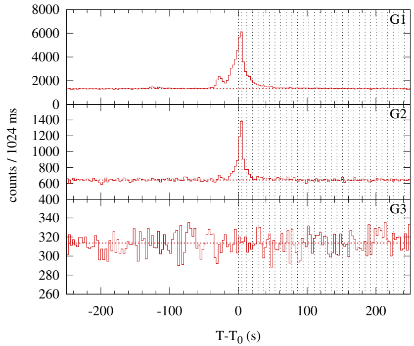
Konus-WIND S2 SOL2000-11-22T16:19 (C7.0) T 0 = 58780.109 s UT (16:19:40.109)
