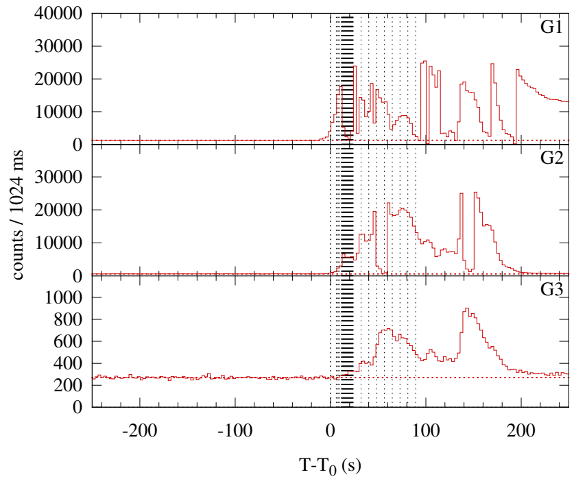
Konus-WIND S2 SOL2000-11-24T04:58 (X2.0) T_0 = 17935.602 s UT (04:58:55.602)
