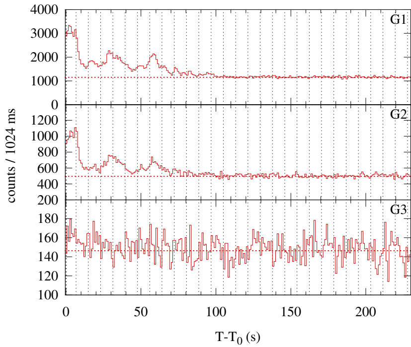
Konus-WIND S2 SOL2000-12-19T10:23 (C9.5) T 0 = 37391.698 s UT (10:23:11.698)
