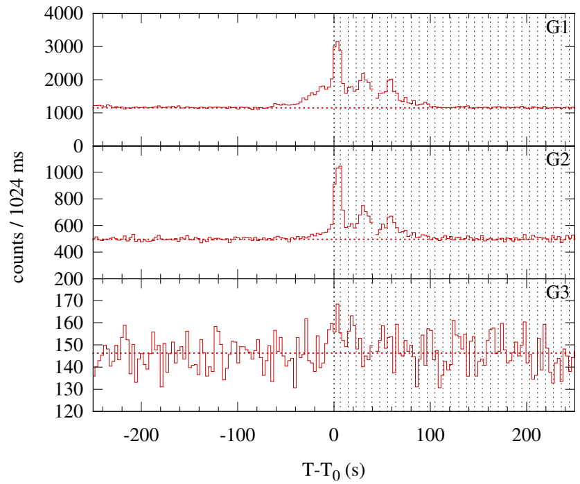
Konus-WIND S2 SOL2000-12-19T10:23 (C9.5) T 0 = 37391.698 s UT (10:23:11.698)
