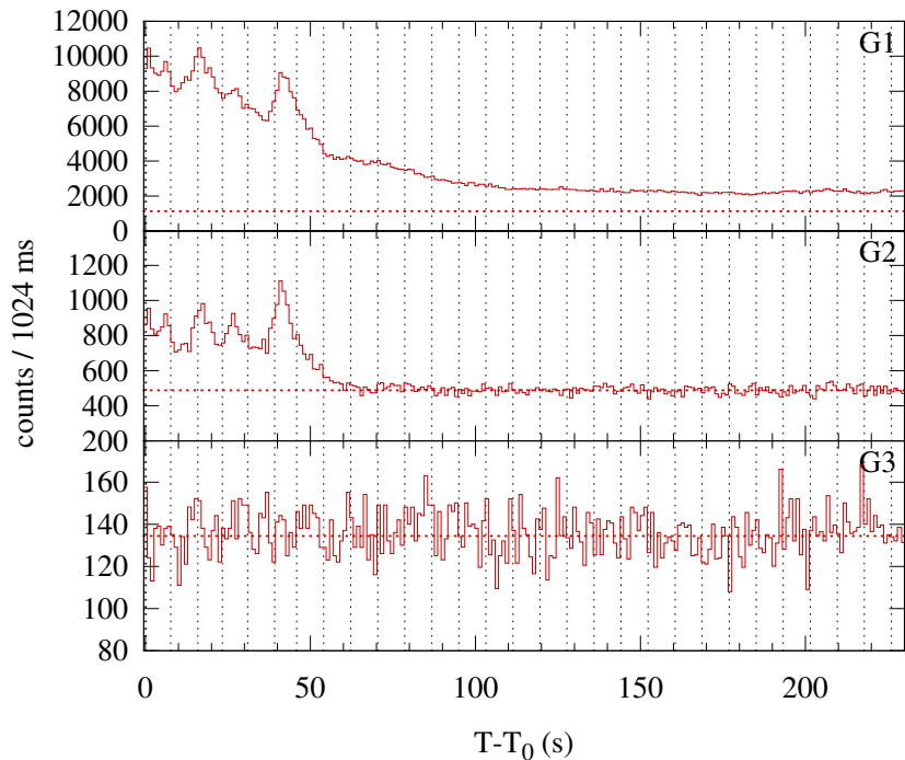
Konus-WIND S2 SOL2000-12-27T15:39 (M4.3) T_0 = 56373.211 s UT (15:39:33.211)
