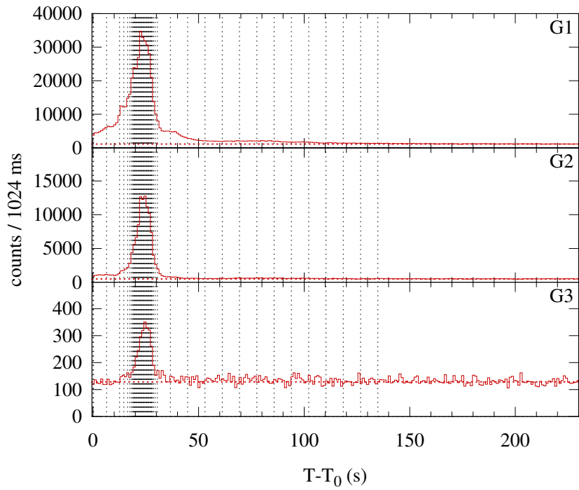
Konus-WIND S2 SOL2001-01-10T10:14 (M3.5) T_0 = 36893.612 s UT (10:14:53.612)
