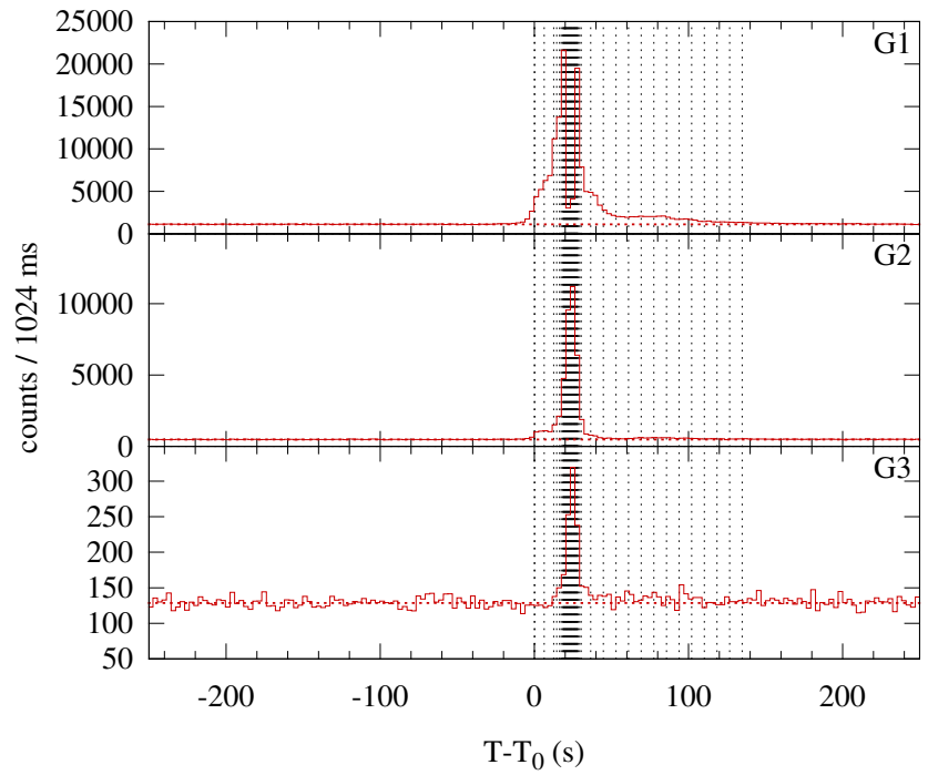
Konus-WIND S2 SOL2001-01-10T10:14 (M3.5) T_0 = 36893.612 s UT (10:14:53.612)
