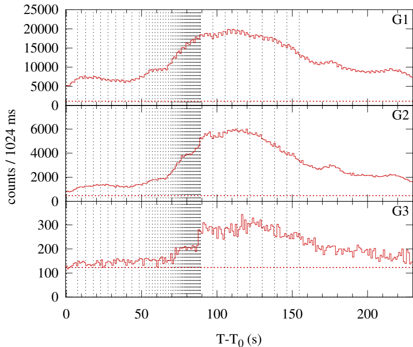
Konus-WIND S2 SOL2001-01-20T21:10 (M7.7) T_0 = 76222.455 s UT (21:10:22.455)
