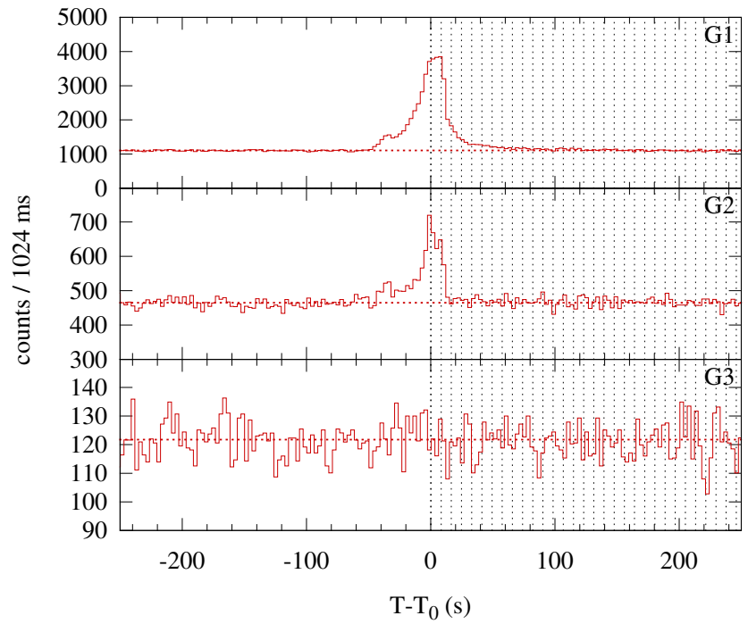
Konus-WIND S2 SOL2001-02-01T07:10 (C7.9) T_0 = 25843.573 s UT (07:10:43.573)
