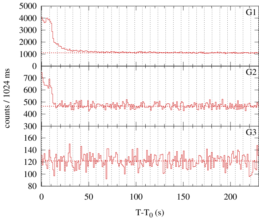
Konus-WIND S2 SOL2001-02-01T07:10 (C7.9) T_0 = 25843.573 s UT (07:10:43.573)
