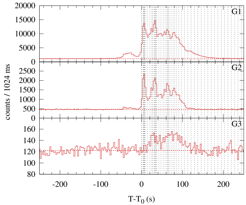
Konus-WIND S2 SOL2001-03-08T11:16 (M5.7) T_0 = 40605.905 s UT (11:16:45.905)
