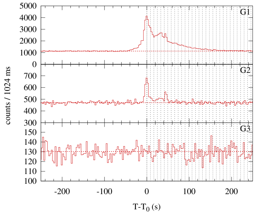
Konus-WIND S2 SOL2001-03-09T01:55 (M1.5) T_0 = 6933.952 s UT (01:55:33.952)
