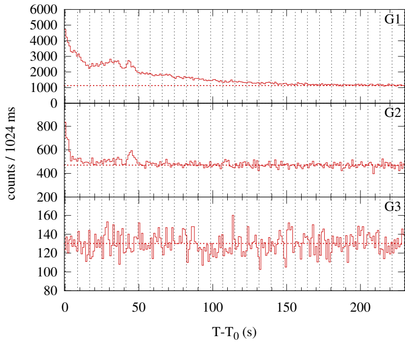
Konus-WIND S2 SOL2001-03-09T01:55 (M1.5) T_0 = 6933.952 s UT (01:55:33.952)
