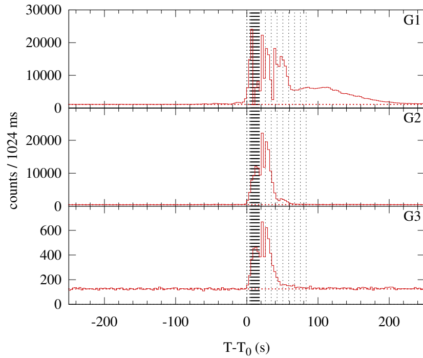
Konus-WIND S2 SOL2001-03-10T04:03 (M6.7) T_0 = 14598.92 s UT (04:03:18.92)
