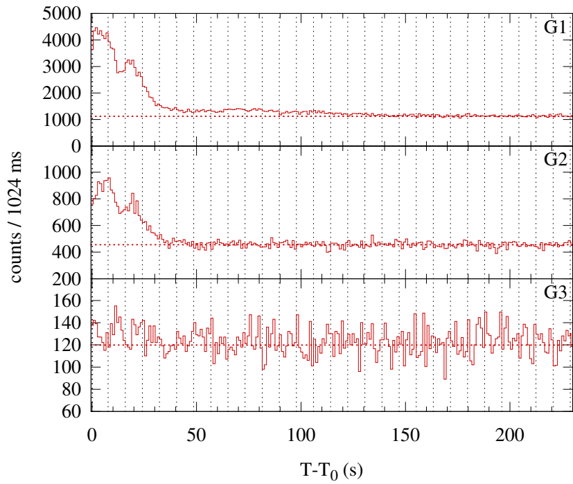
Konus-WIND S2 SOL2001-03-21T11:25 (C9.8) T_0 = 41112.343 s UT (11:25:12.343)
