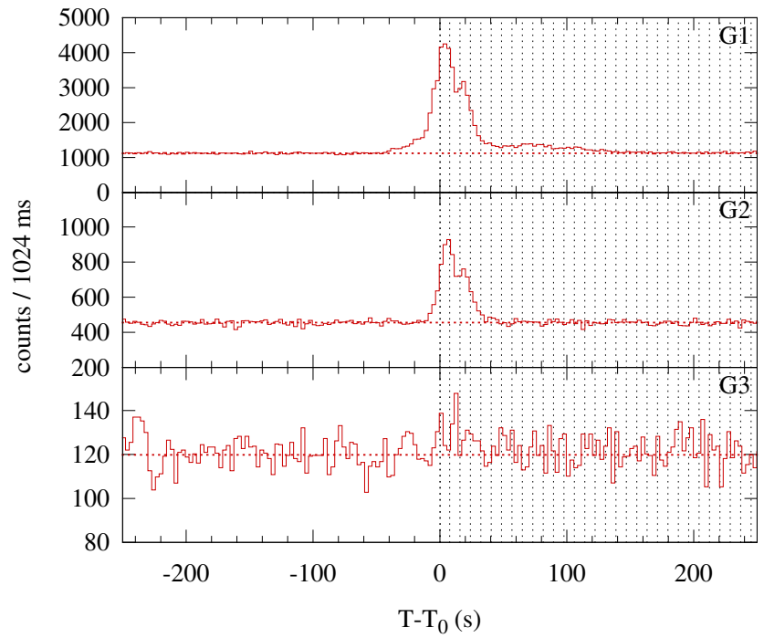
Konus-WIND S2 SOL2001-03-21T11:25 (C9.8) T_0 = 41112.343 s UT (11:25:12.343)
