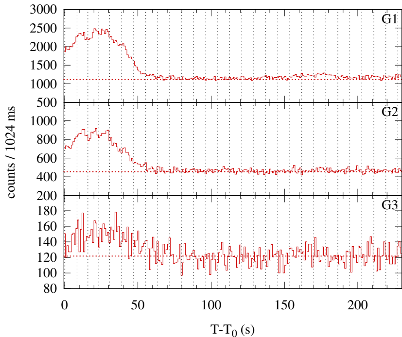
Konus-WIND S2 SOL2001-03-24T01:35 (M1.2) T 0 = 5709.234 s UT (01:35:09.234)
