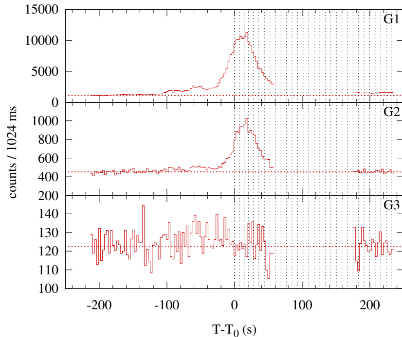
Konus-WIND S2 SOL2001-03-25T04:17 (M2.5) T 0 = 15443.214 s UT (04:17:23.214)
