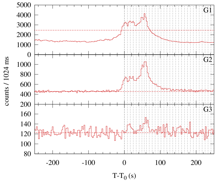
Konus-WIND S2 SOL2001-03-25T11:14 (M2.6) T 0 = 40484.954 s UT (11:14:44.954)
