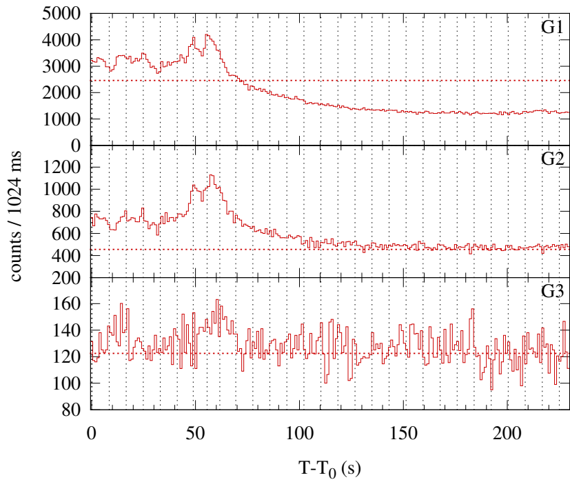
Konus-WIND S2 SOL2001-03-25T11:14 (M2.6) T 0 = 40484.954 s UT (11:14:44.954)
