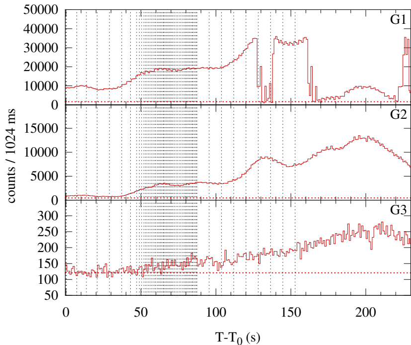
Konus-WIND S2 SOL2001-03-29T10:03 (X1.7) T_0 = 36199.694 s UT (10:03:19.694)
