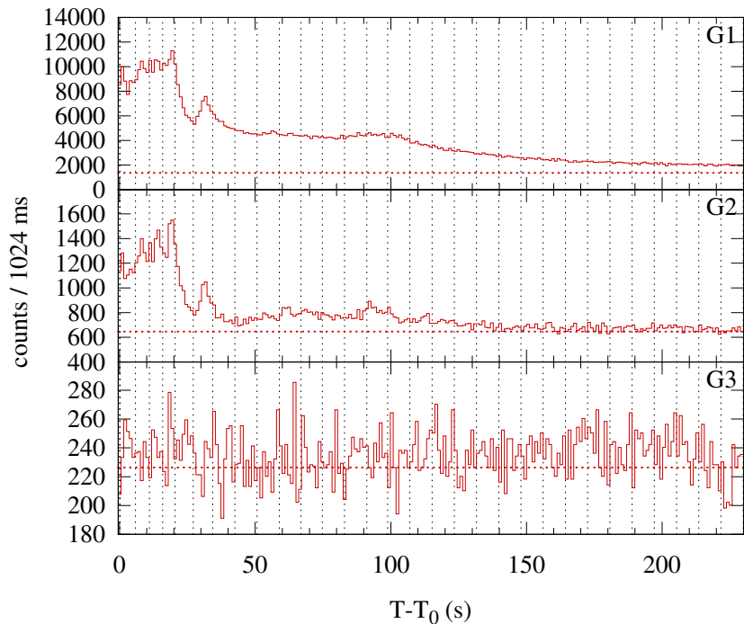
Konus-WIND S2 SOL2001-04-02T00:17 (M3.2) T 0 = 1040.514 s UT (00:17:20.514)
