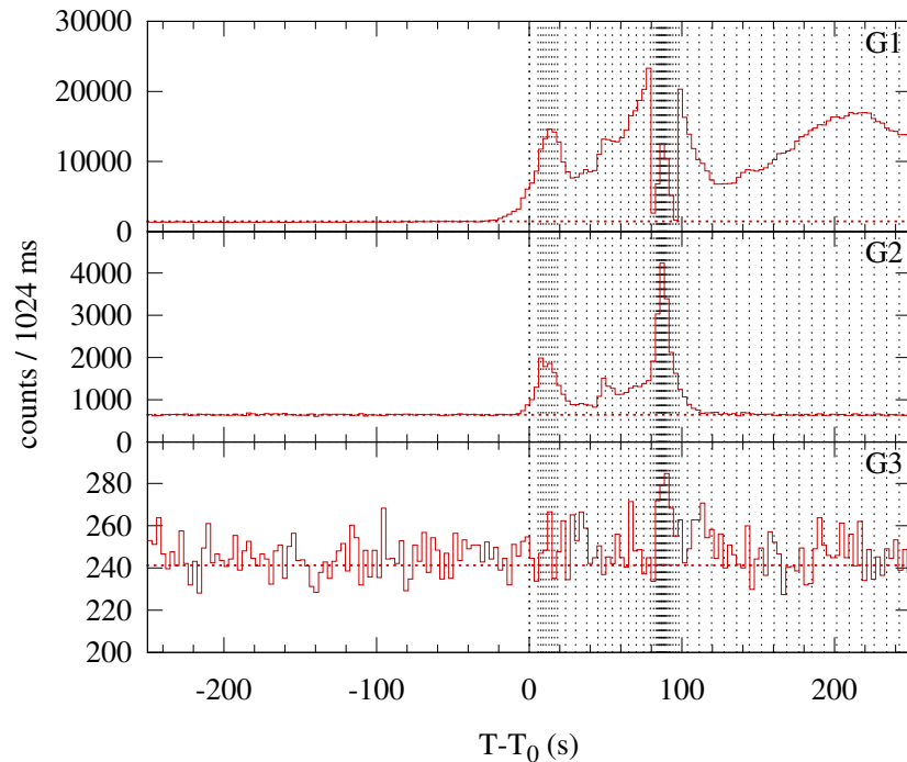
Konus-WIND S2 SOL2001-04-02T10:06 (X1.4) T 0 = 36360.142 s UT (10:06:00.142)
