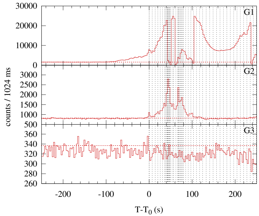
Konus-WIND S2 SOL2001-04-02T21:34 (X20) T 0 = 77695.783 s UT (21:34:55.783)
