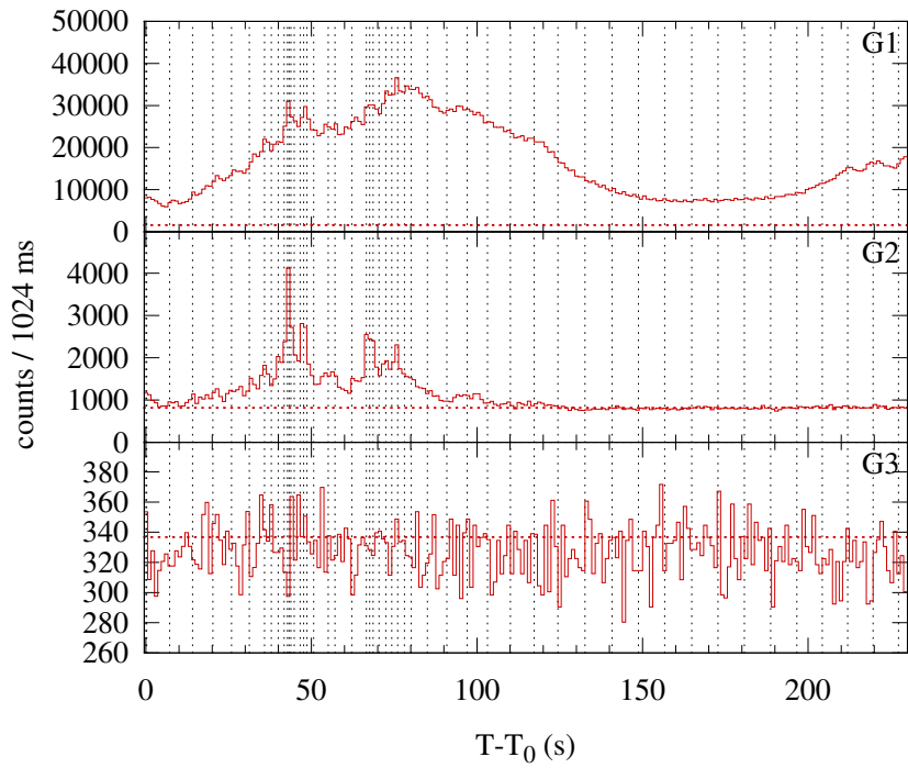
Konus-WIND S2 SOL2001-04-02T21:34 (X20) T 0 = 77695.783 s UT (21:34:55.783)
