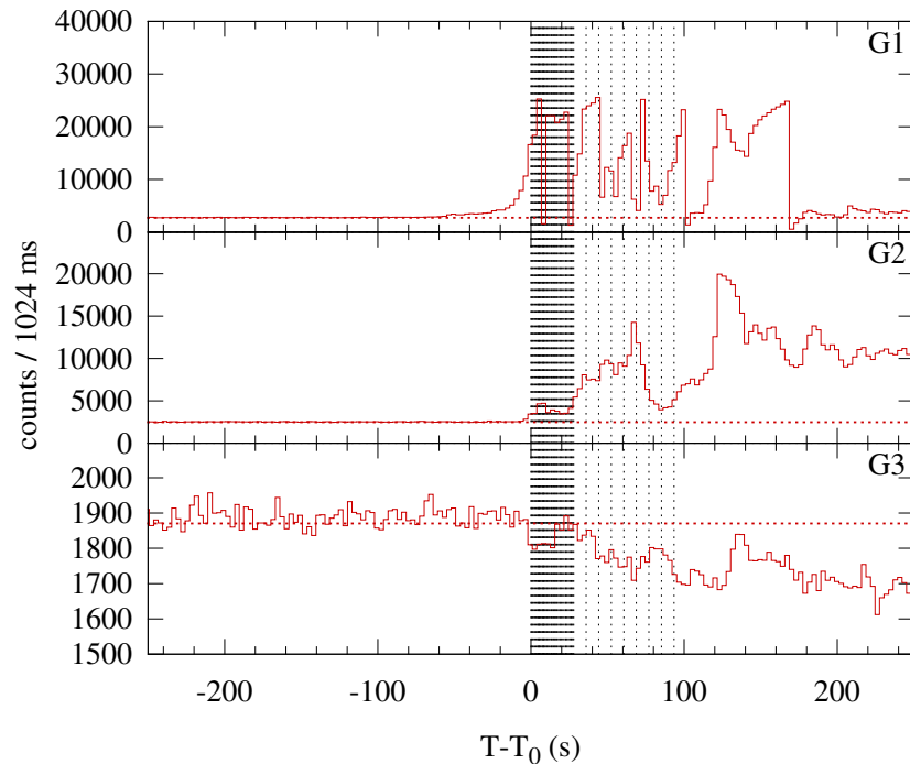
Konus-WIND S2 SOL2001-04-06T19:13 (X5.6) T_0 = 69215.472 s UT (19:13:35.472)
