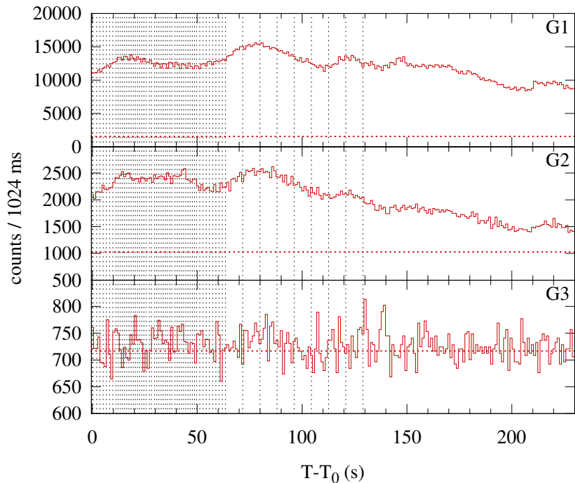
Konus-WIND S2 SOL2001-04-10T05:12 (X2.3) T_0 = 18748.362 s UT (05:12:28.362)
