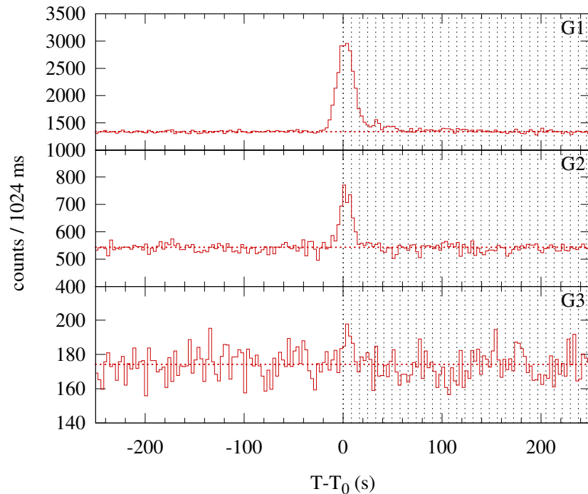
Konus-WIND S2 SOL2001-04-15T04:06 (C2.2) T_0 = 14763.211 s UT (04:06:03.211)
