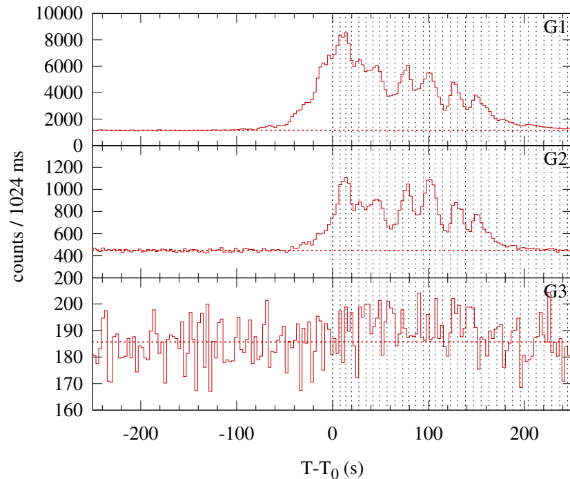
Konus-WIND S2 SOL2001-04-22T20:40 (M3.2) T_0 = 74425.90 s UT (20:40:25.90)
