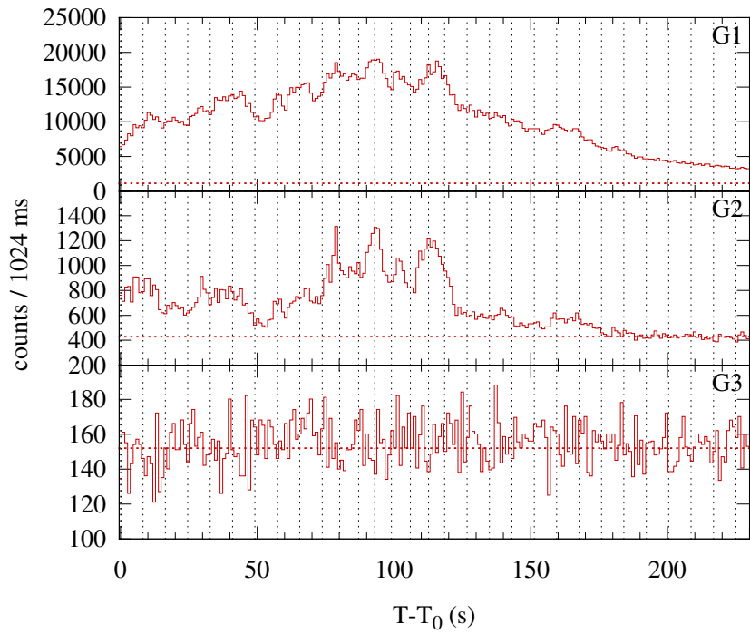
Konus-WIND S2 SOL2001-04-26T13:08 (M7.8) T 0 = 47294.519 s UT (13:08:14.519)
