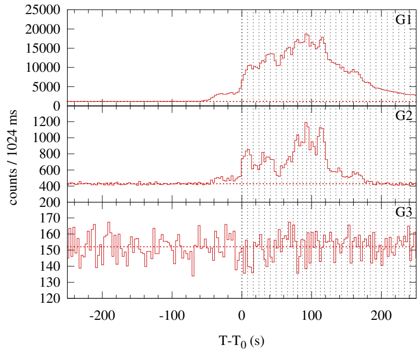
Konus-WIND S2 SOL2001-04-26T13:08 (M7.8) T 0 = 47294.519 s UT (13:08:14.519)
