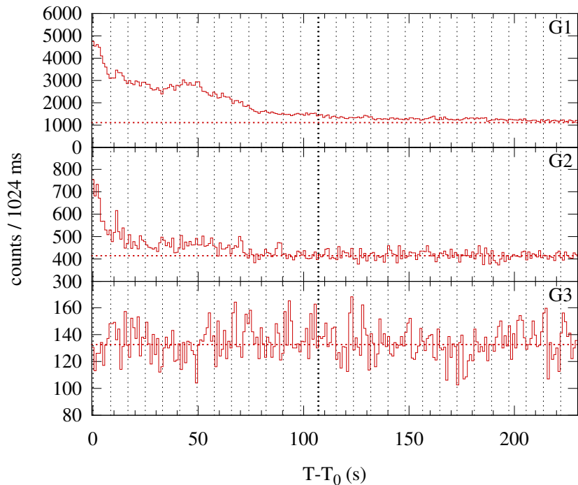
Konus-WIND S2 SOL2001-05-02T00:36 (M1.8) T_0 = 2160.240 s UT (00:36:00.240)
