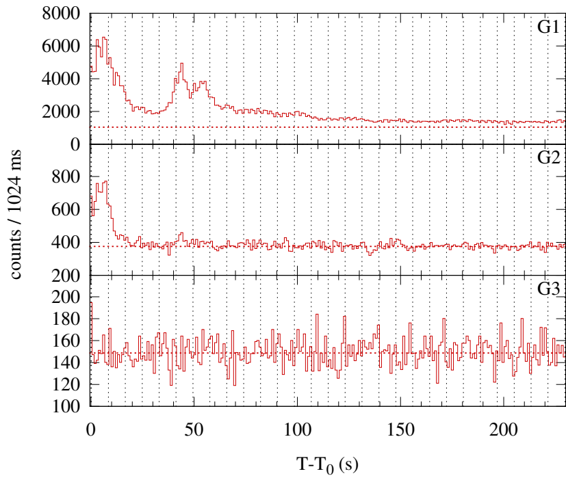
Konus-WIND S1 SOL2001-05-12T23:27 (M3.0) T_0 = 84444.736 s UT (23:27:24.736)
