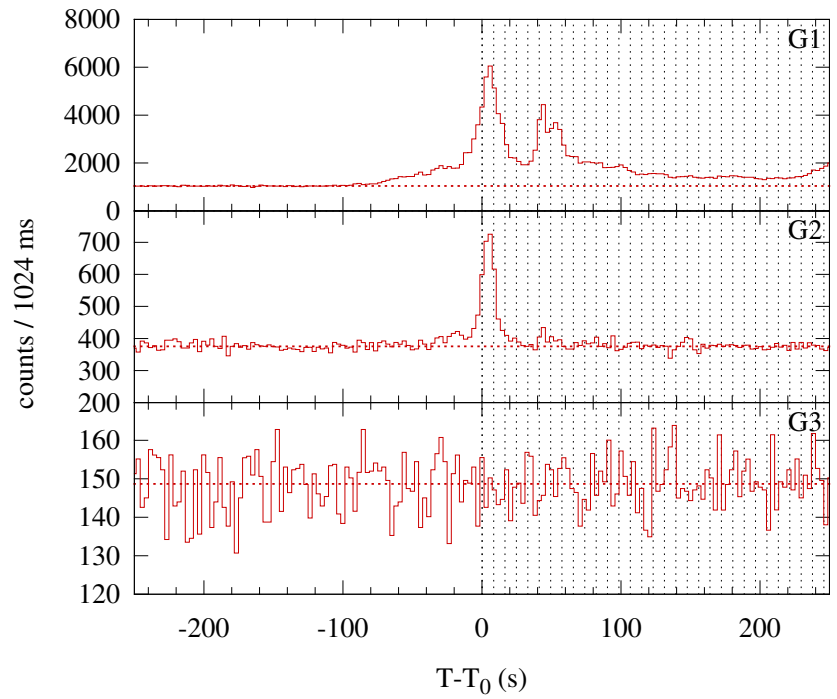
Konus-WIND S1 SOL2001-05-12T23:27 (M3.0) T_0 = 84444.736 s UT (23:27:24.736)
