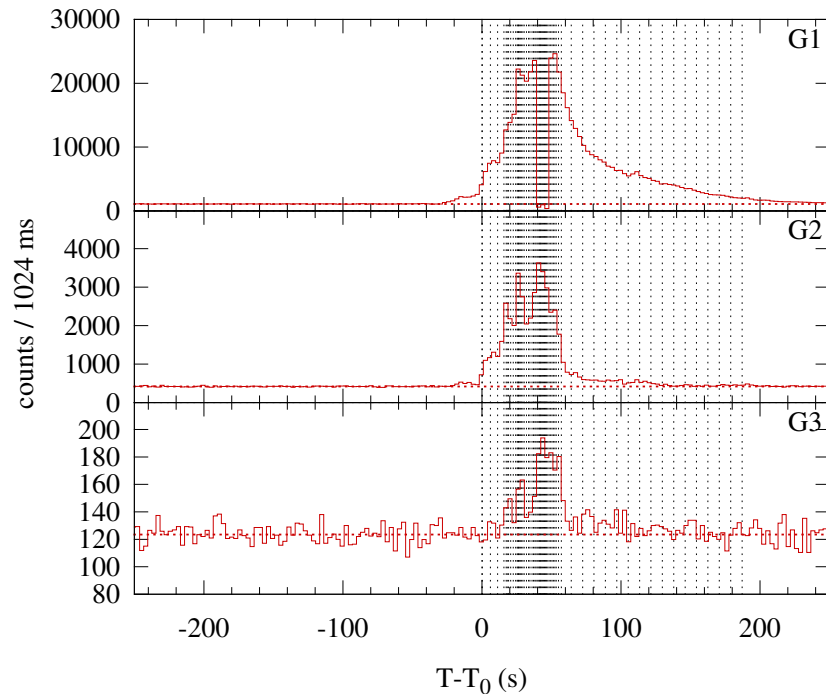
Konus-WIND S2 SOL2001-05-20T06:01 (M6.4) T_0 = 21712.605 s UT (06:01:52.605)
