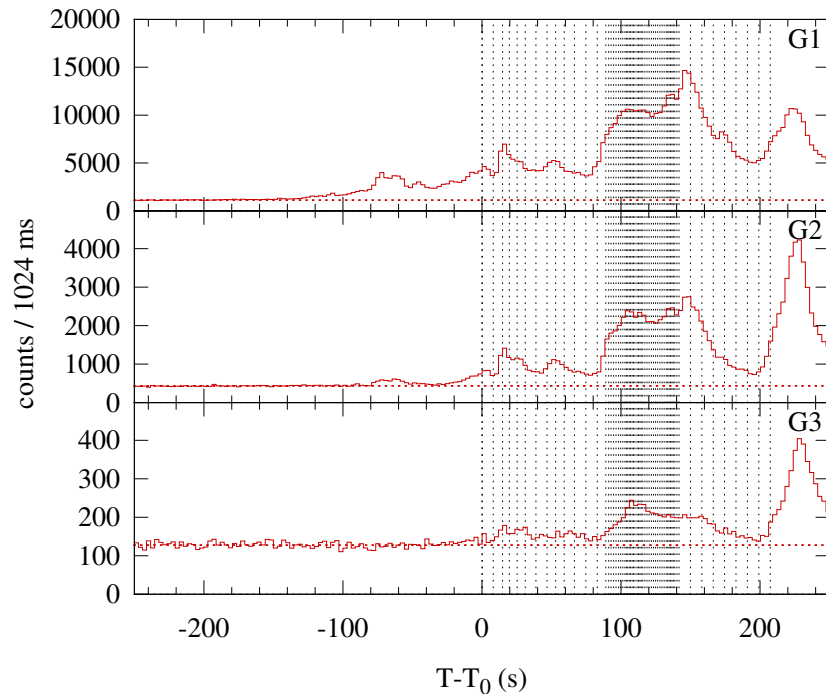
Konus-WIND S2 SOL2001-06-13T11:36 (M7.8) T_0 = 41812.168 s UT (11:36:52.168)
