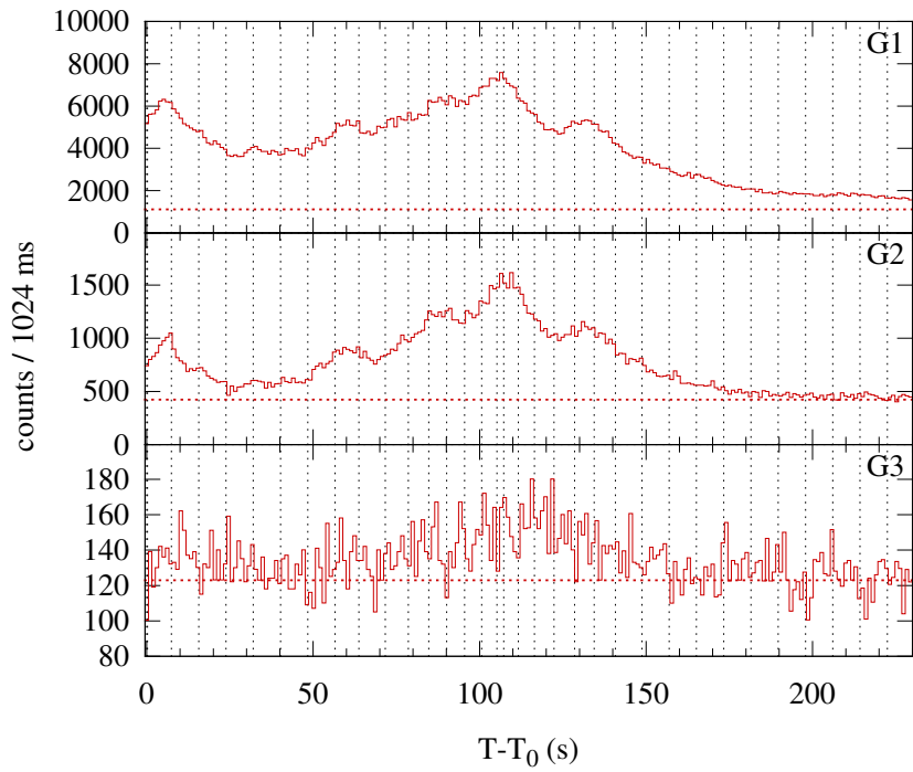
Konus-WIND S2 SOL2001-06-15T10:11 (M6.3) T_0 = 36677.561 s UT (10:11:17.561)
