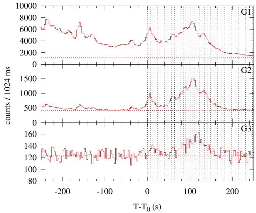
Konus-WIND S2 SOL2001-06-15T10:11 (M6.3) T_0 = 36677.561 s UT (10:11:17.561)
