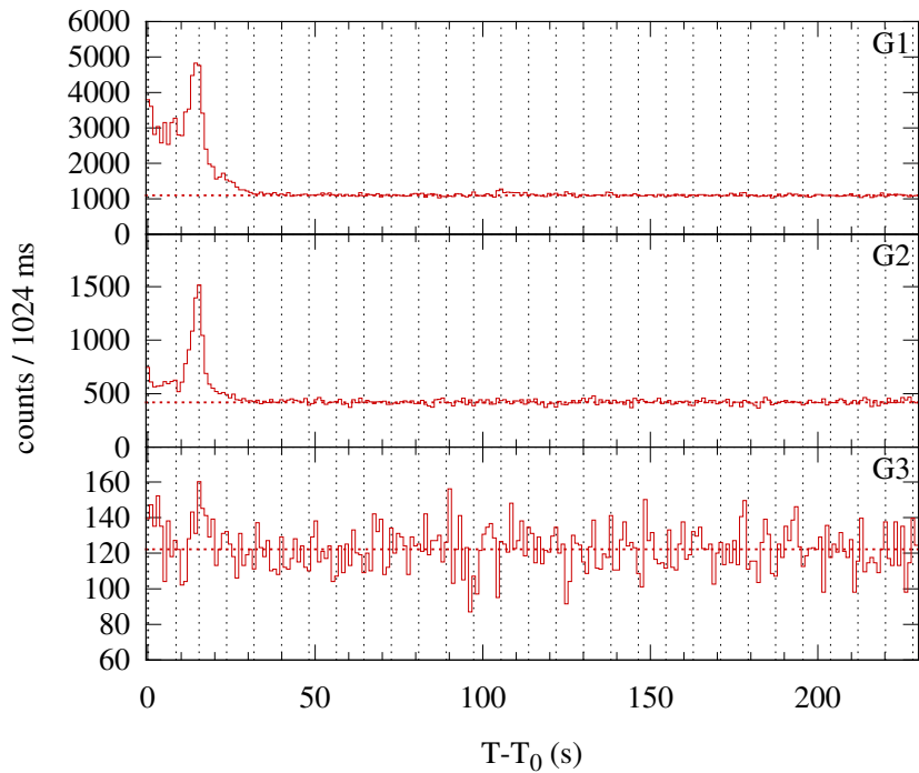
Konus-WIND S2 SOL2001-06-24T03:13 (C2.9) T 0 = 11607.353 s UT (03:13:27.353)
