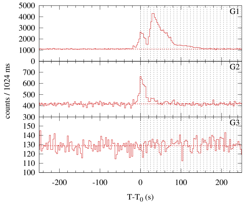
Konus-WIND S2 SOL2001-08-03T03:05 (M1.5) T 0 = 11139.704 s UT (03:05:39.704)
