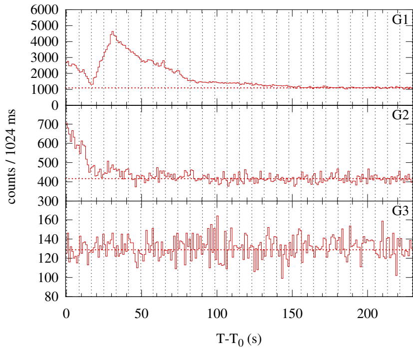
Konus-WIND S2 SOL2001-08-03T03:05 (M1.5) T 0 = 11139.704 s UT (03:05:39.704)
