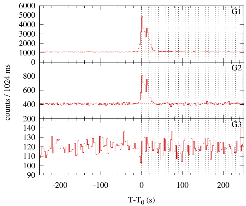
Konus-WIND S2 SOL2001-08-05T15:03 (C3.5) T_0 = 54213.20 s UT (15:03:33.20)
