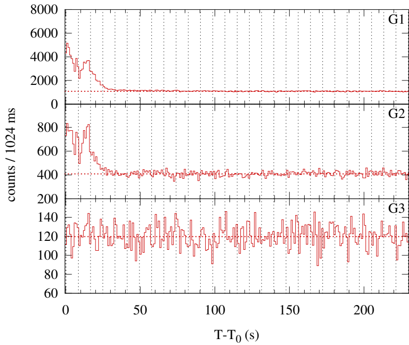
Konus-WIND S2 SOL2001-08-05T15:03 (C3.5) T_0 = 54213.20 s UT (15:03:33.20)
