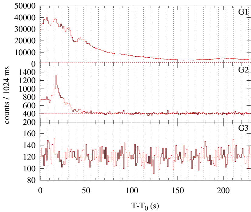
Konus-WIND S2 SOL2001-08-05T22:19 (M4.9) T 0 = 80399.162 s UT (22:19:59.162)
