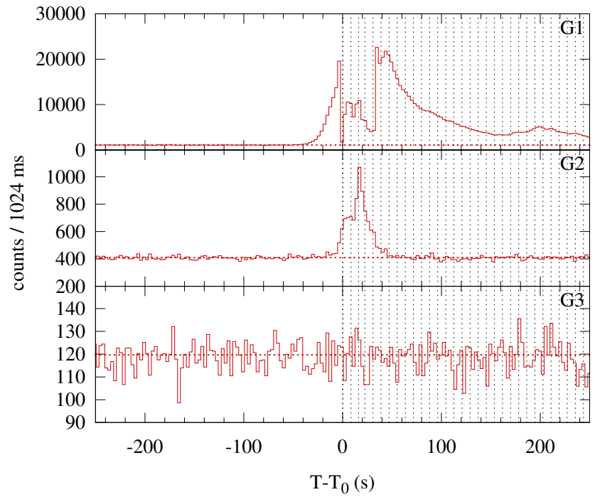
Konus-WIND S2 SOL2001-08-05T22:19 (M4.9) T 0 = 80399.162 s UT (22:19:59.162)
