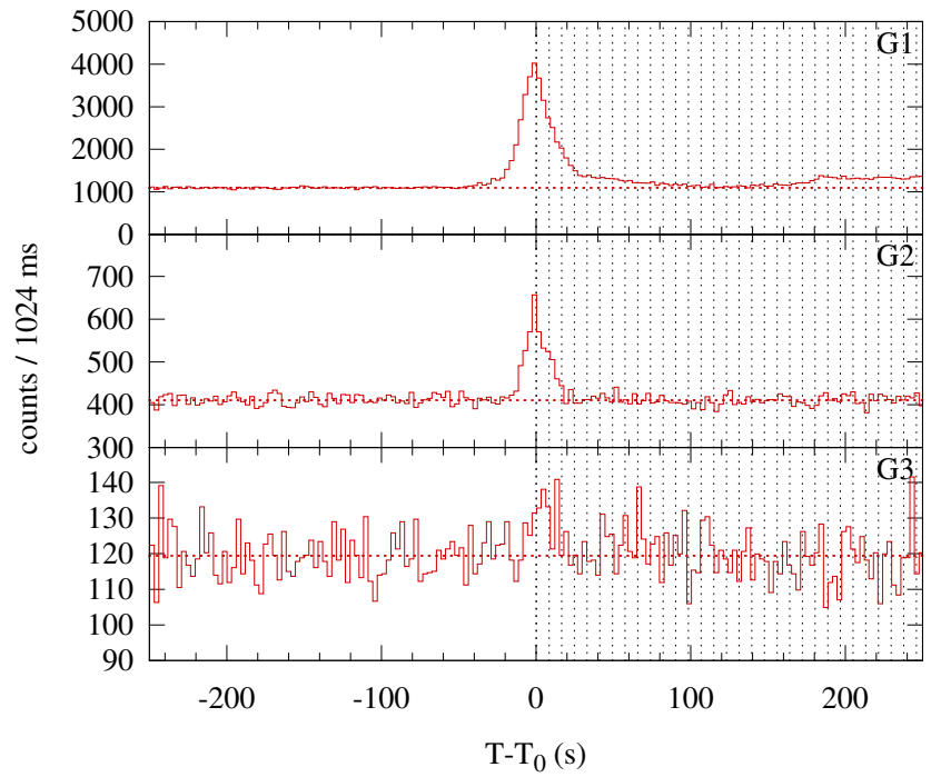
Konus-WIND S2 SOL2001-08-07T07:29 (M1.1) T_0 = 26943.481 s UT (07:29:03.481)
