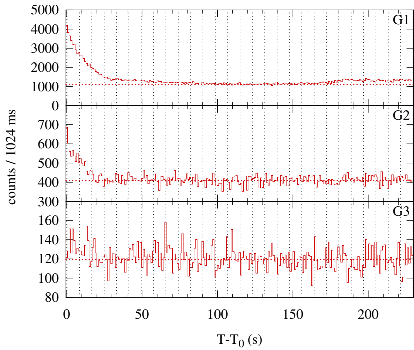
Konus-WIND S2 SOL2001-08-07T07:29 (M1.1) T_0 = 26943.481 s UT (07:29:03.481)
