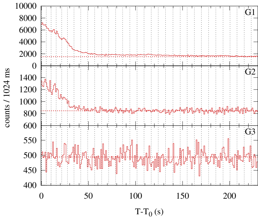
Konus-WIND S2 SOL2001-08-21T21:55 (M1.5) T_0 = 78900.351 s UT (21:55:00.351)
