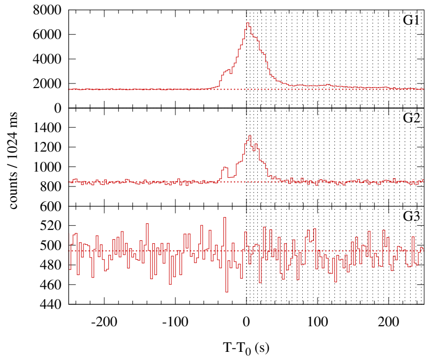
Konus-WIND S2 SOL2001-08-21T21:55 (M1.5) T_0 = 78900.351 s UT (21:55:00.351)
