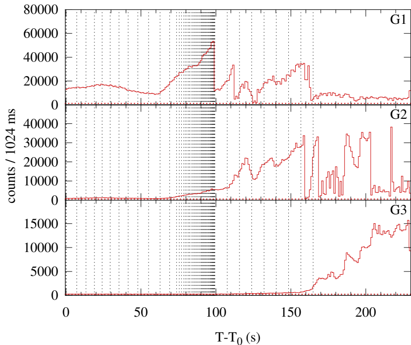
Konus-WIND S2 SOL2001-08-25T16:28 (X5.3) T 0 = 59284.57 s UT (16:28:04.57)
