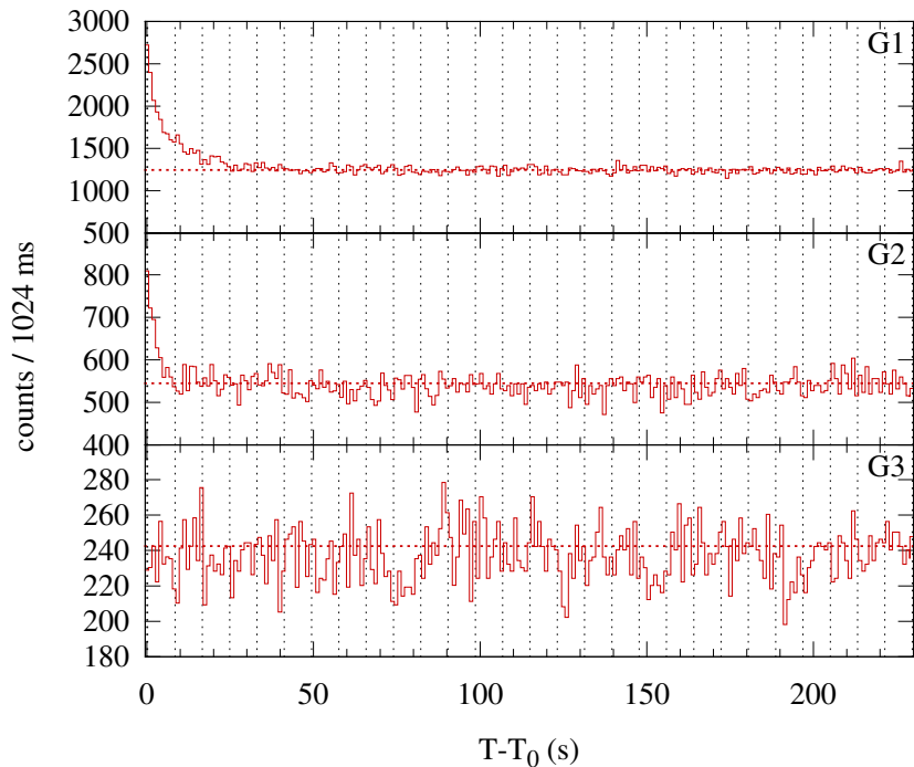
Konus-WIND S2 SOL2001-08-25T19:55 (M1.19) T 0 = 71758.39 s UT (19:55:58.39)
