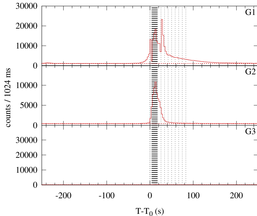
Konus-WIND S2 SOL2001-08-30T20:35 (M3.0) T 0 = 74159.86 s UT (20:35:59.86)
