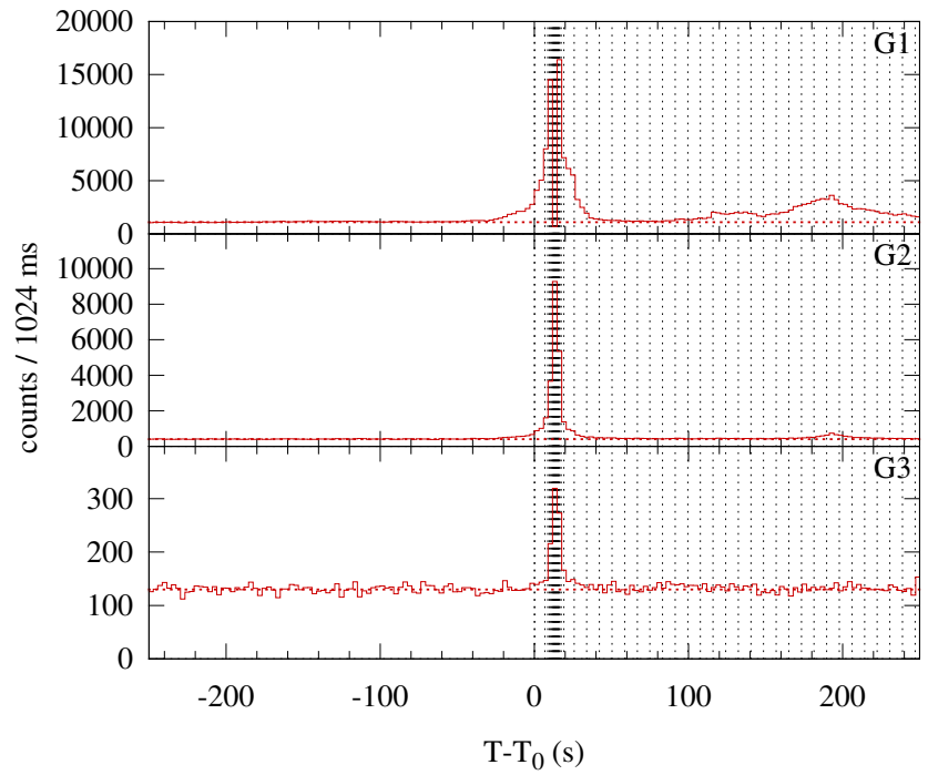
Konus-WIND S2 SOL2001-08-31T10:37 (M1.6) T_0 = 38278.531 s UT (10:37:58.531)
