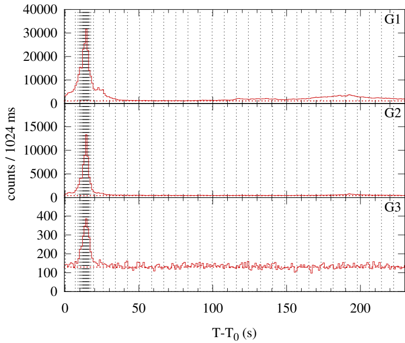
Konus-WIND S2 SOL2001-08-31T10:37 (M1.6) T_0 = 38278.531 s UT (10:37:58.531)
