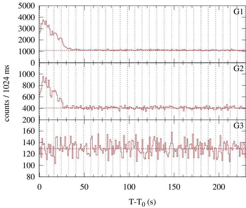
Konus-WIND S2 SOL2001-09-01T20:41 (C2.7) T_0 = 74488.115 s UT (20:41:28.115)
