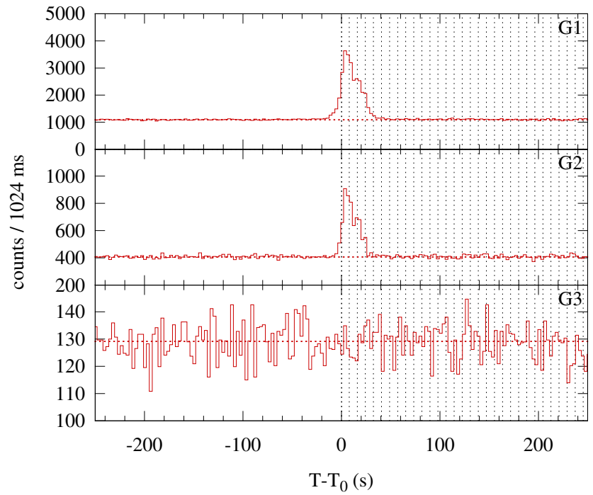
Konus-WIND S2 SOL2001-09-01T20:41 (C2.7) T_0 = 74488.115 s UT (20:41:28.115)
