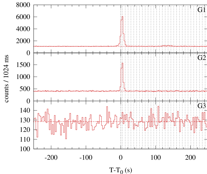
Konus-WIND S2 SOL2001-09-02T05:43 (C2.1) T 0 = 20615.109 s UT (05:43:35.109)
