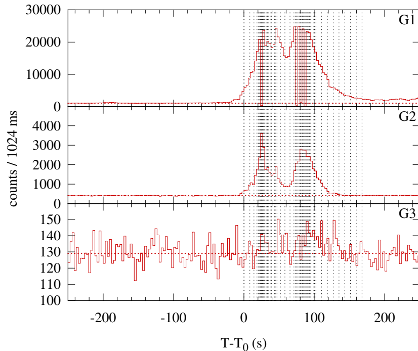
Konus-WIND S2 SOL2001-09-02T13:45 (M3.0) T_0 = 49510.778 s UT (13:45:10.778)
