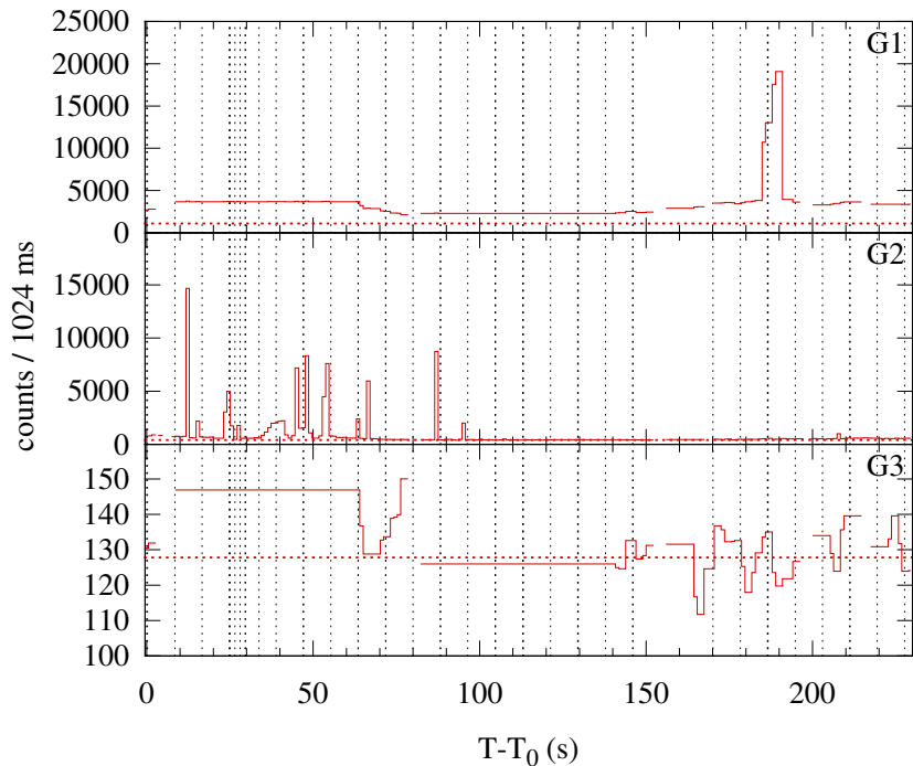
Konus-WIND S2 SOL2001-09-05T14:27 (M6.0) T_0 = 52062.338 s UT (14:27:42.338)
