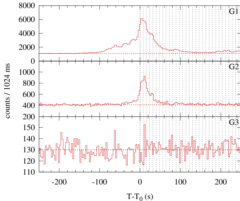
Konus-WIND S2 SOL2001-09-07T15:29 (M1.2) T 0 = 55783.14 s UT (15:29:43.14)
